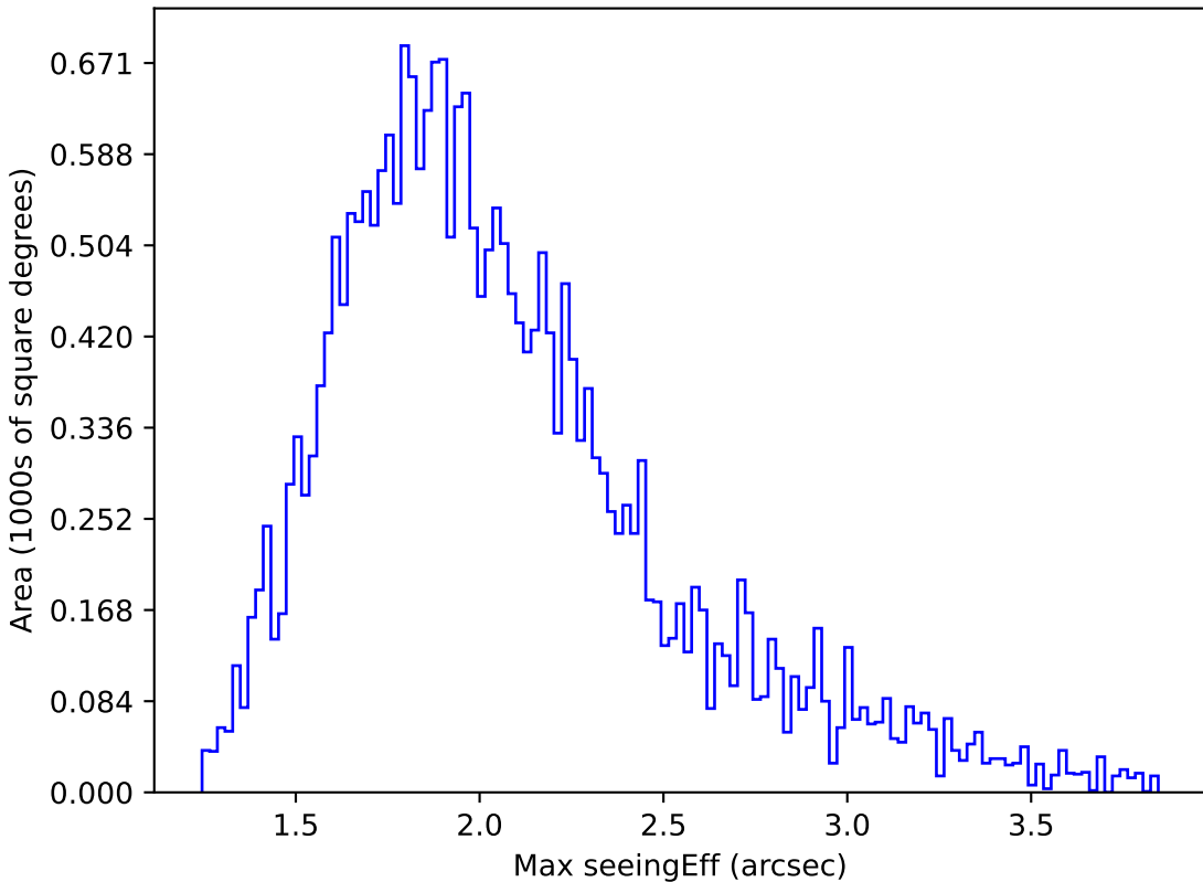
too_ignore_100_1v3.4_10yrs Yr 1 all bands: Max seeingEff
