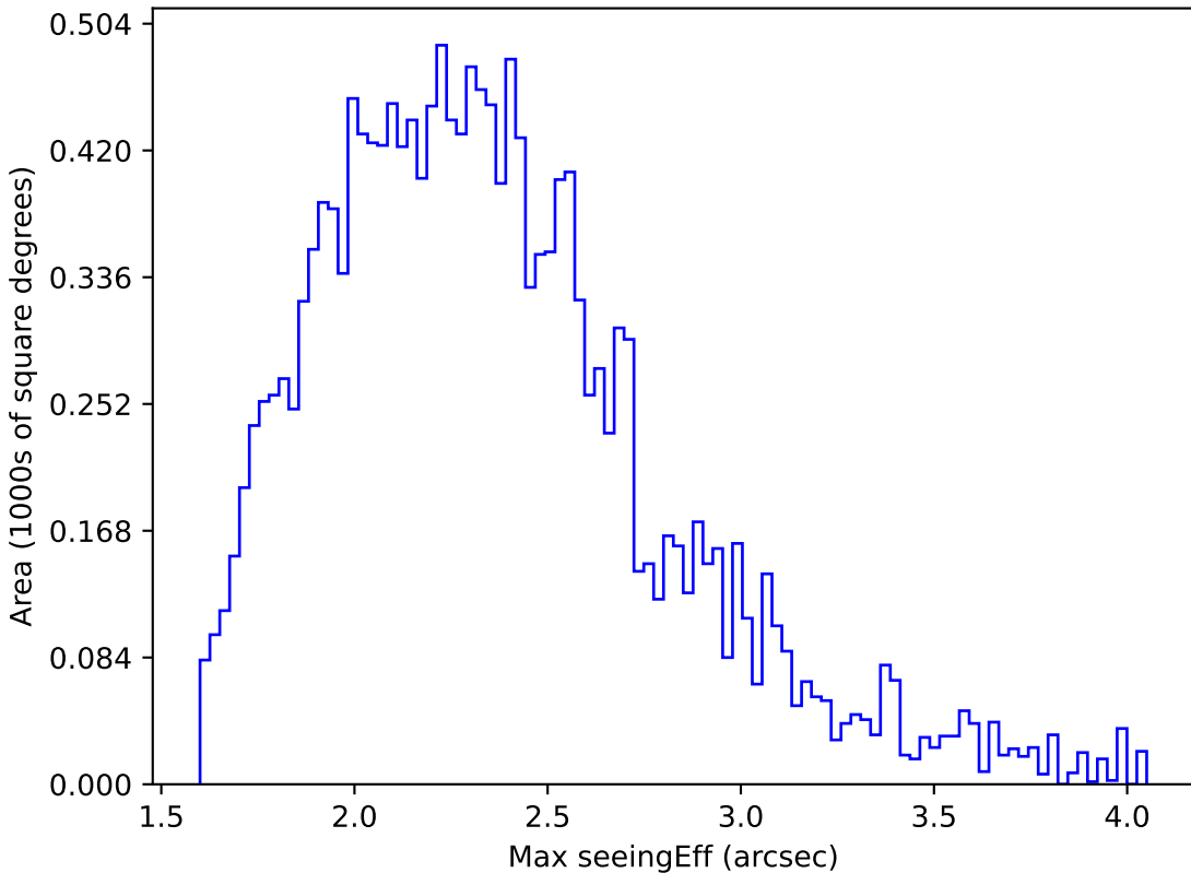
too_ignore_100_1v3.4_10yrs WFD y band: Max seeingEff
