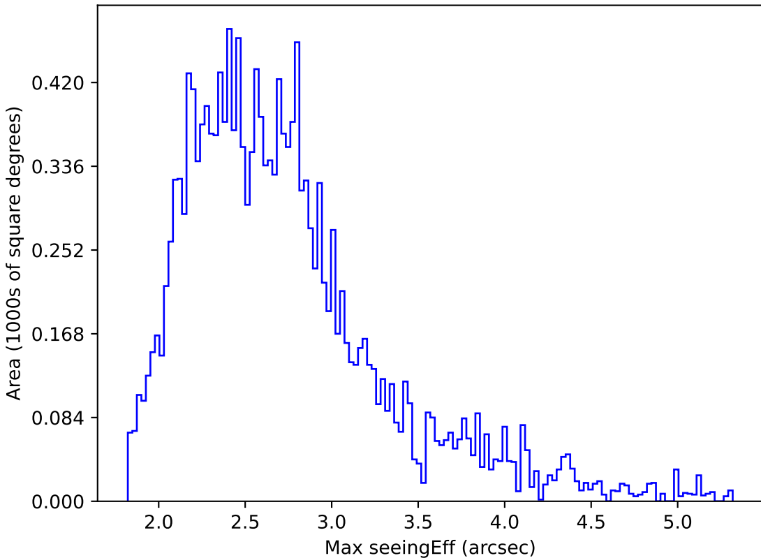
too_ignore_100_1v3.4_10yrs WFD r band: Max seeingEff
