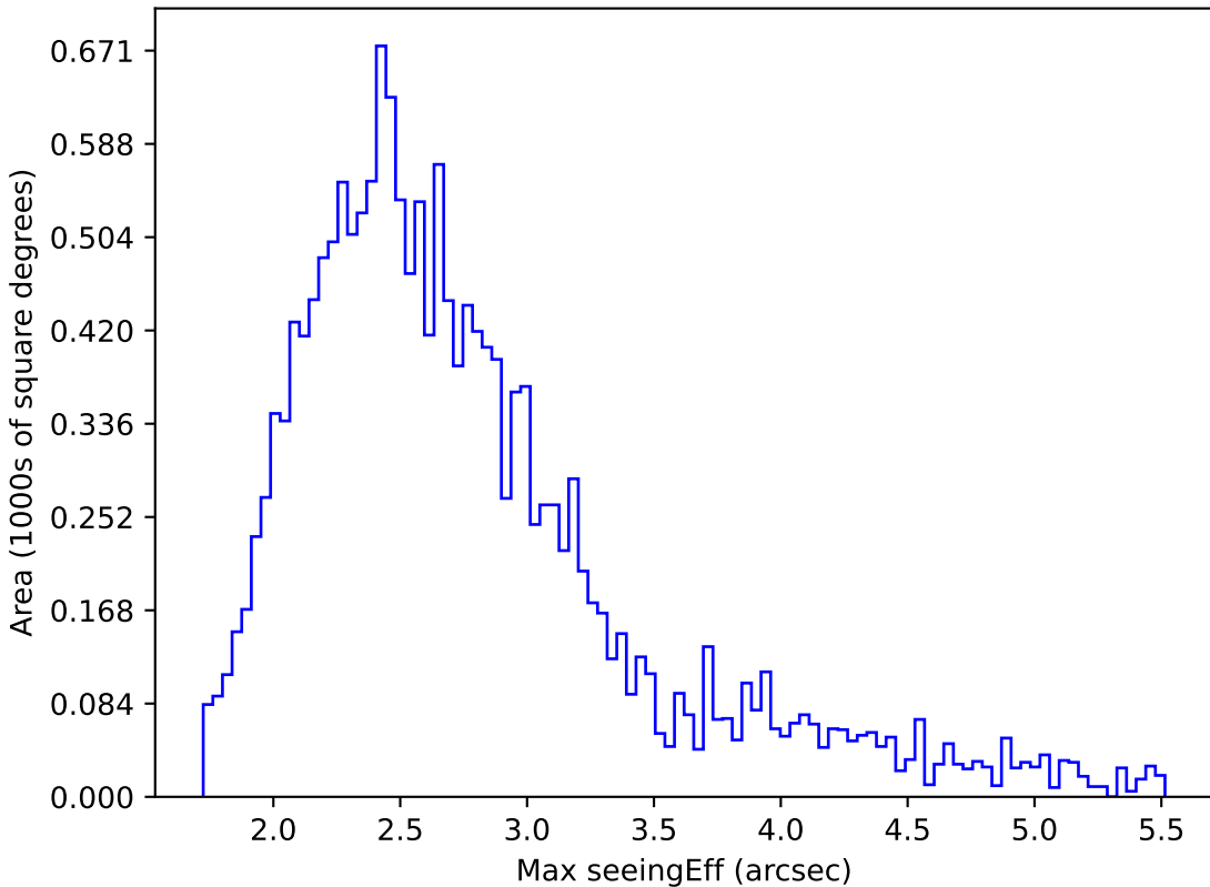
too_ignore_100_1v3.4_10yrs WFD i band: Max seeingEff
