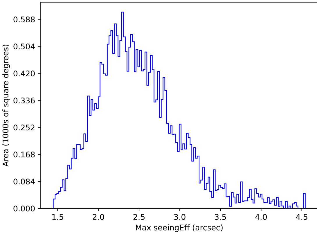
too_ignore_100_1v3.4_10yrs All sky z band: Max seeingEff
