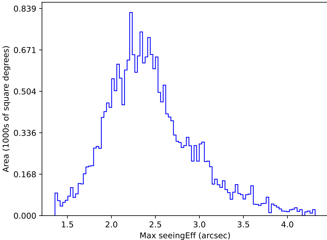
too_ignore_100_1v3.4_10yrs All sky u band: Max seeingEff
