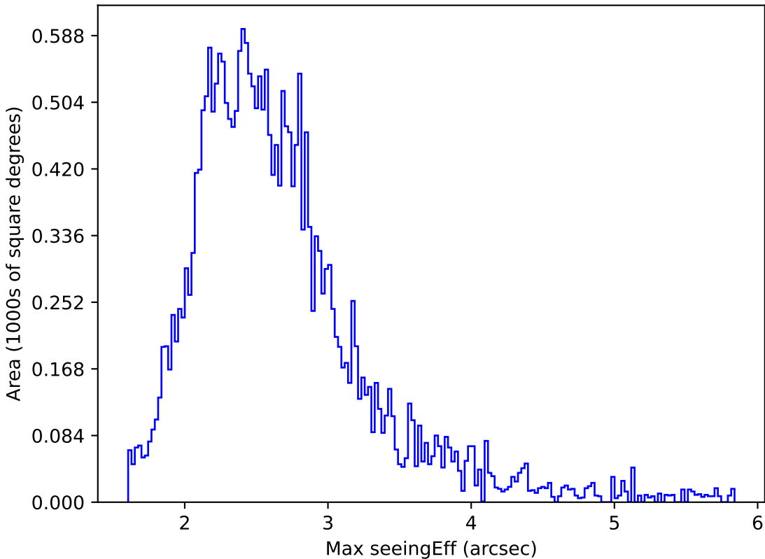
too_ignore_100_1v3.4_10yrs All sky r band: Max seeingEff
