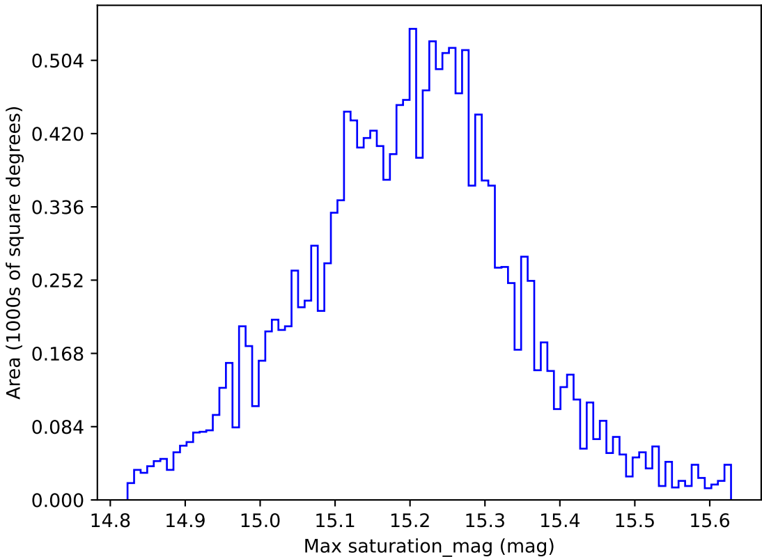
too_ignore_100_1v3.4_10yrs WFD z band: Max saturation_mag
