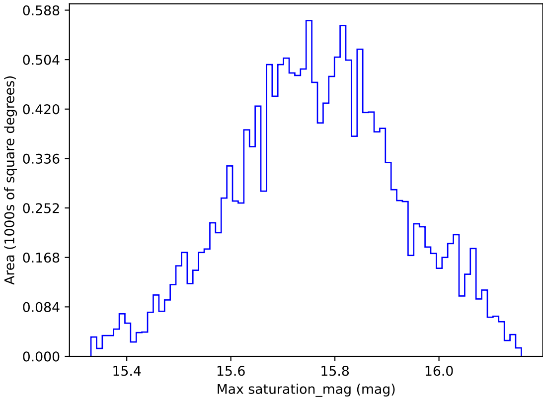
too_ignore_100_1v3.4_10yrs WFD r band: Max saturation_mag
