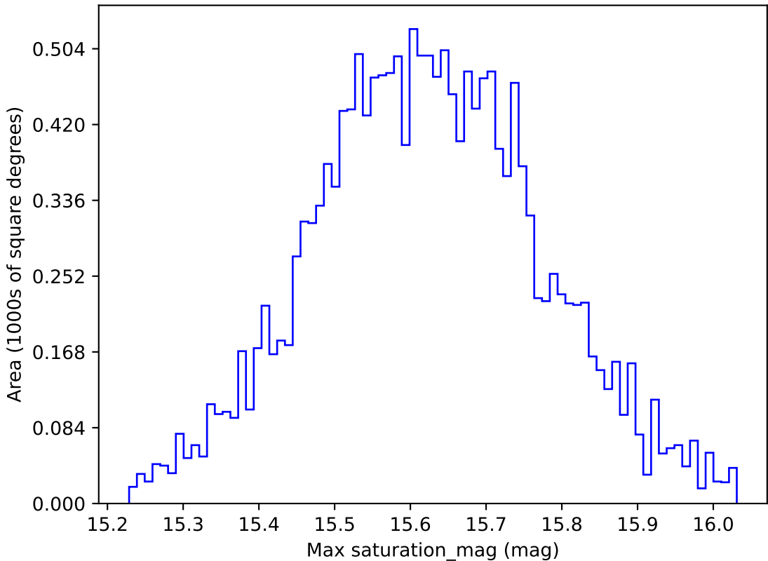
too_ignore_100_1v3.4_10yrs WFD i band: Max saturation_mag
