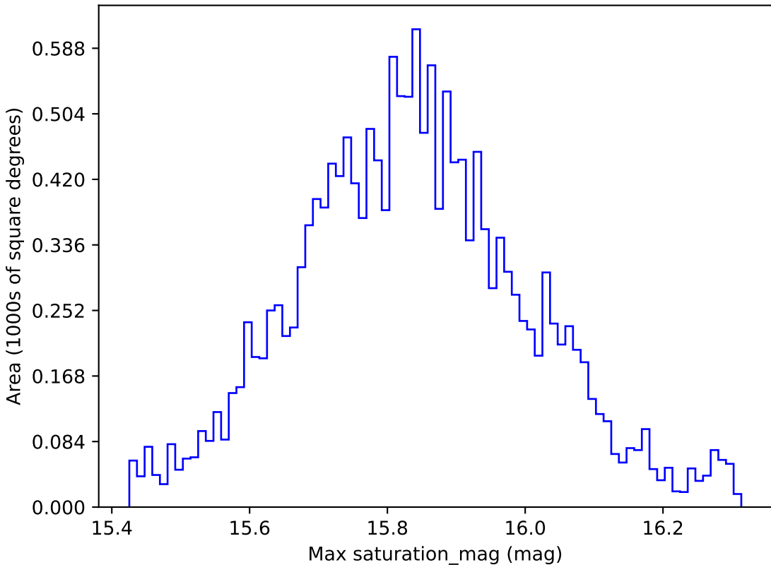
too_ignore_100_1v3.4_10yrs WFD all bands: Max saturation_mag
