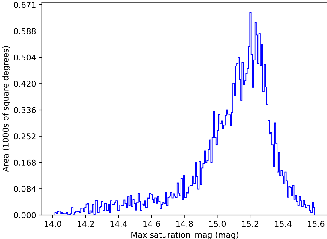
too_ignore_100_1v3.4_10yrs All sky z band: Max saturation_mag
