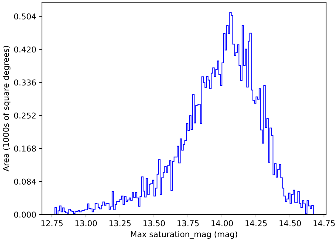
too_ignore_100_1v3.4_10yrs All sky u band: Max saturation_mag
