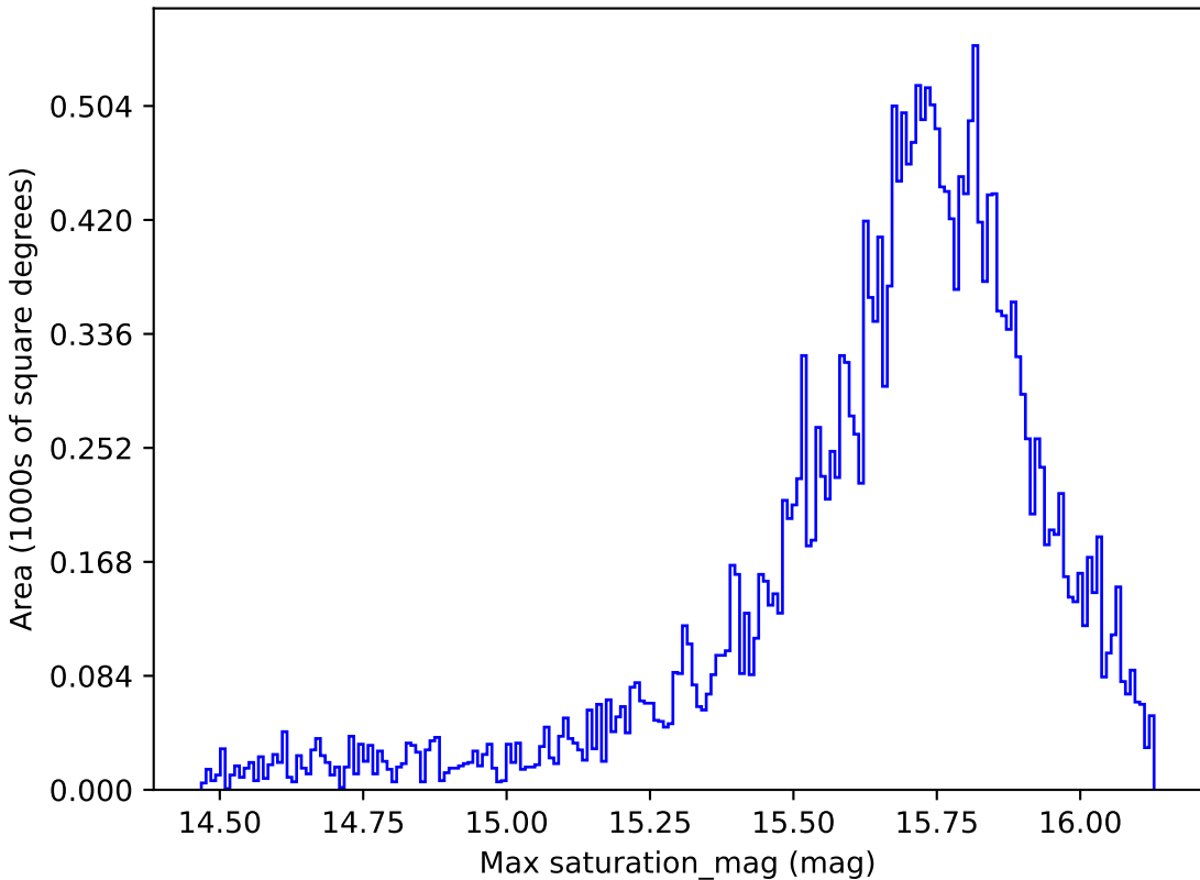
too_ignore_100_1v3.4_10yrs All sky r band: Max saturation_mag
