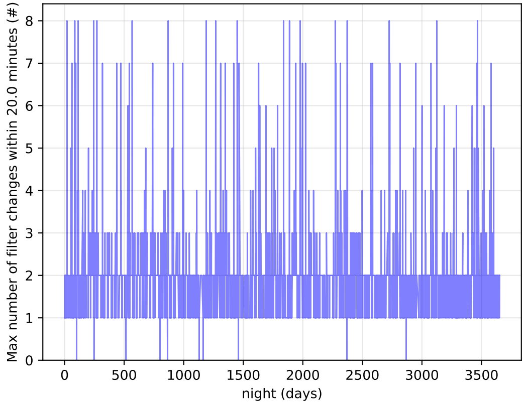
too_ignore_100_1v3.4_10yrs Per Night: Max number of filter changes within 20.0 minutes
