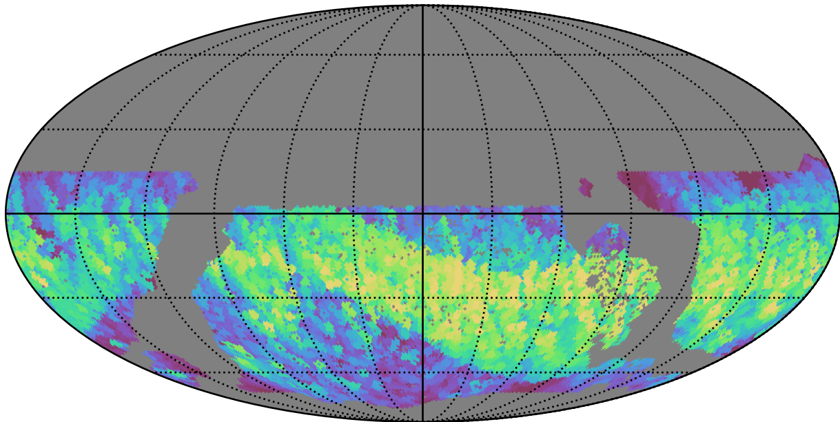
too_ignore_100_1v3.4_10yrs WFD z band: Max normairmass
