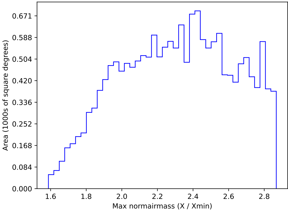
too_ignore_100_1v3.4_10yrs WFD z band: Max normairmass
