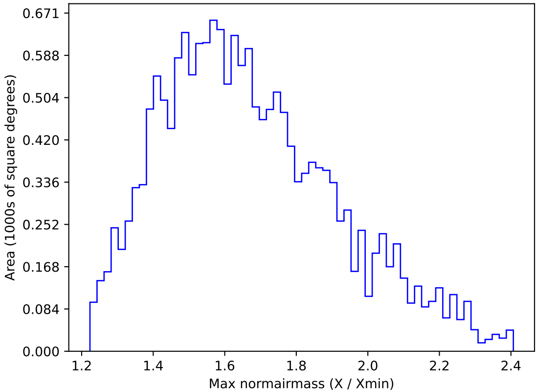
too_ignore_100_1v3.4_10yrs WFD u band: Max normairmass
