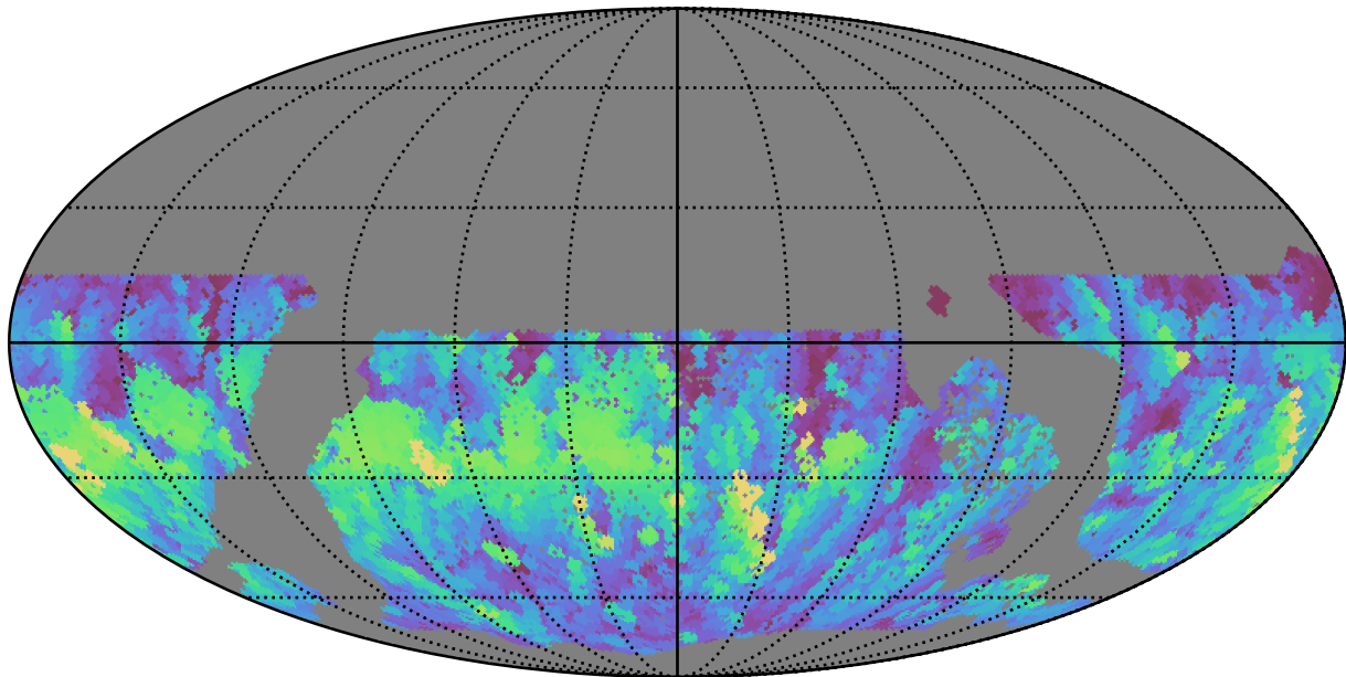
too_ignore_100_1v3.4_10yrs WFD g band: Max normairmass
