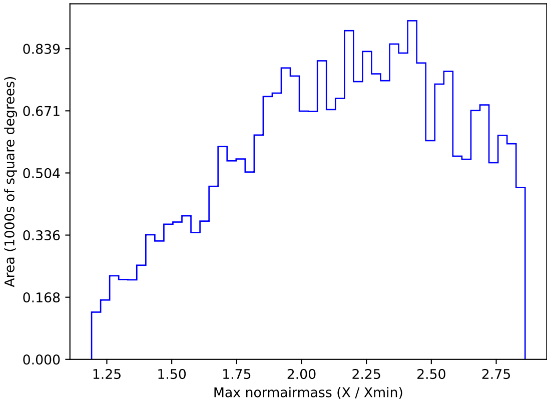
too_ignore_100_1v3.4_10yrs All sky z band: Max normairmass
