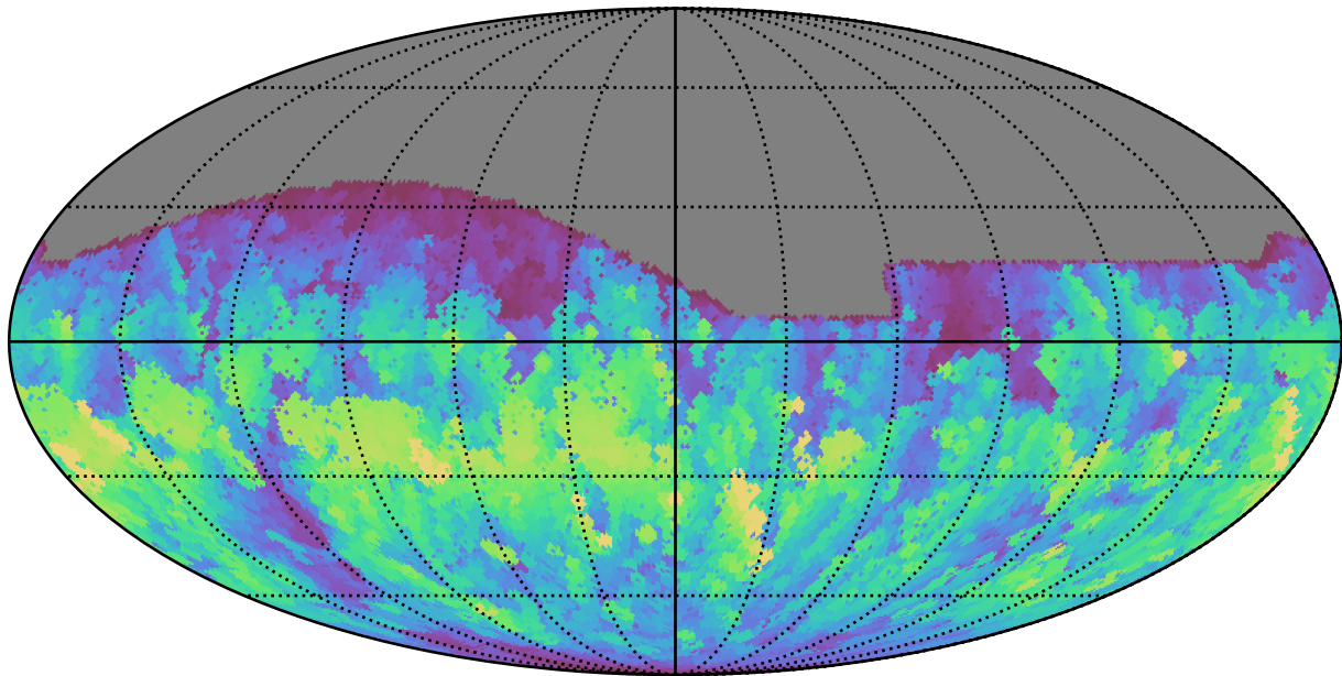
too_ignore_100_1v3.4_10yrs All sky g band: Max normairmass
