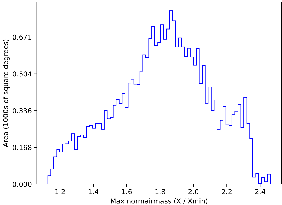
too_ignore_100_1v3.4_10yrs All sky g band: Max normairmass
