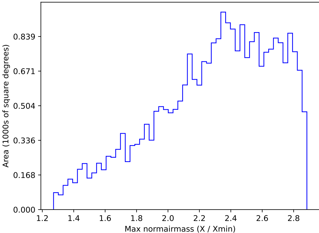
too_ignore_100_1v3.4_10yrs All sky all bands: Max normairmass
