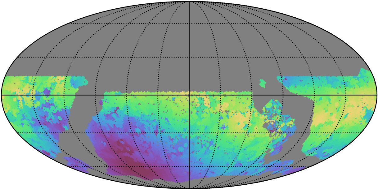
too_ignore_100_1v3.4_10yrs WFD y band: Max moonDistance
