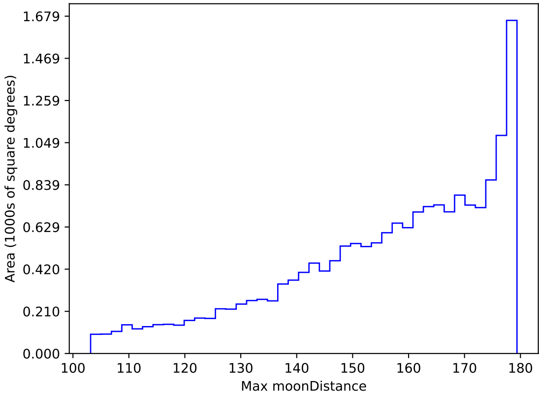
too_ignore_100_1v3.4_10yrs WFD r band: Max moonDistance
