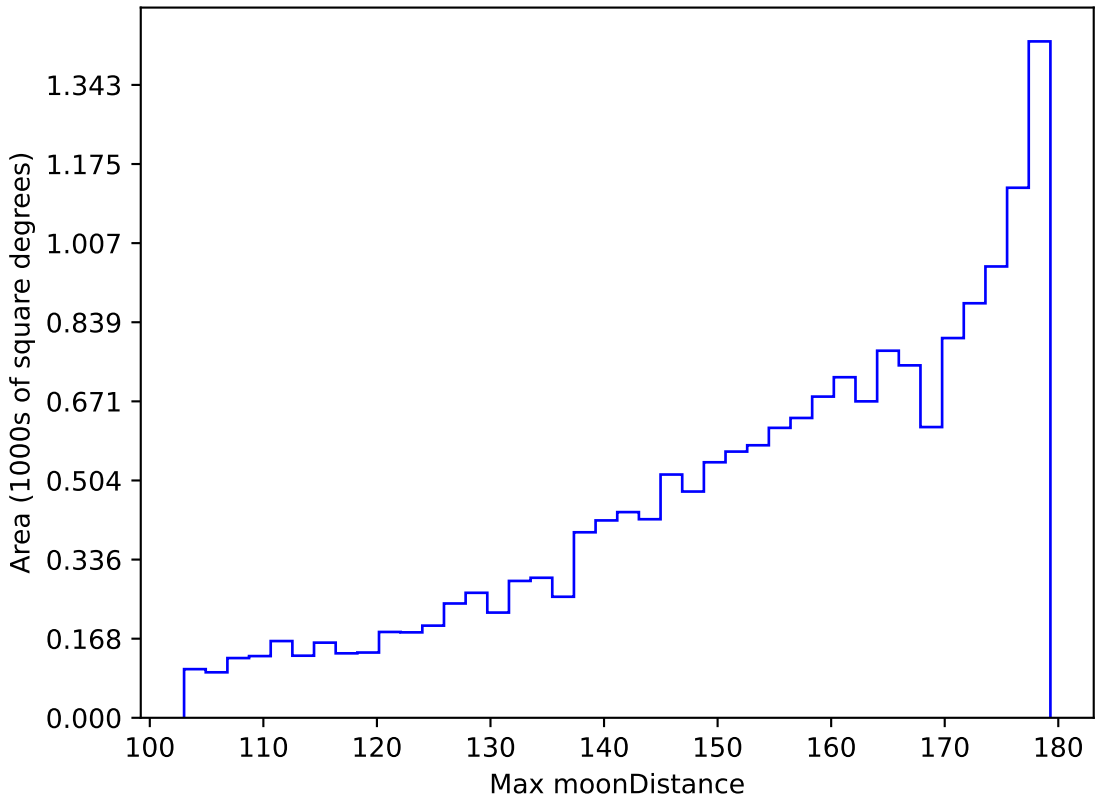
too_ignore_100_1v3.4_10yrs WFD i band: Max moonDistance
