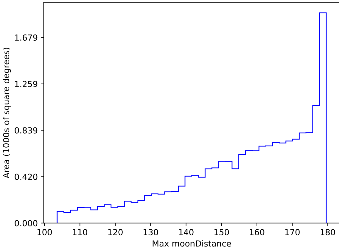
too_ignore_100_1v3.4_10yrs WFD all bands: Max moonDistance
