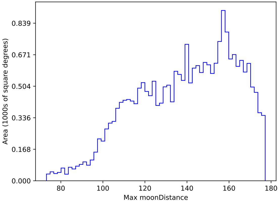
too_ignore_100_1v3.4_10yrs All sky y band: Max moonDistance
