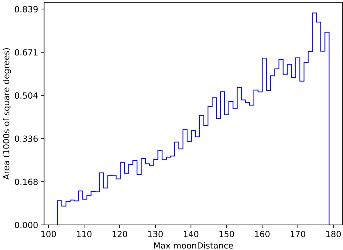
too_ignore_100_1v3.4_10yrs All sky u band: Max moonDistance
