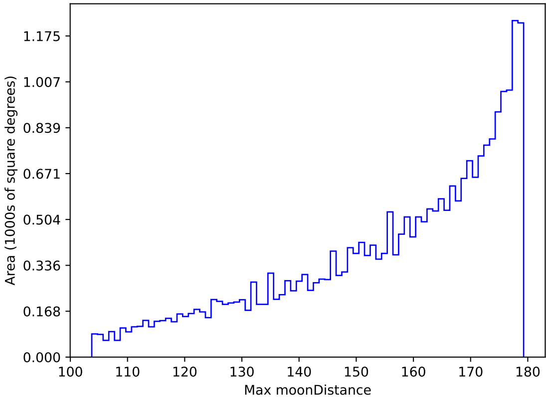
too_ignore_100_1v3.4_10yrs All sky r band: Max moonDistance
