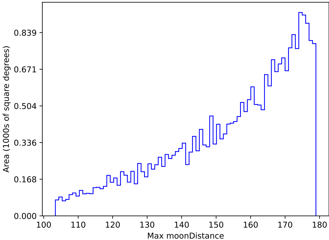
too_ignore_100_1v3.4_10yrs All sky g band: Max moonDistance
