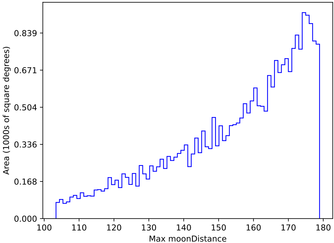
too_ignore_100_1v3.4_10yrs All sky g band: Max moonDistance
