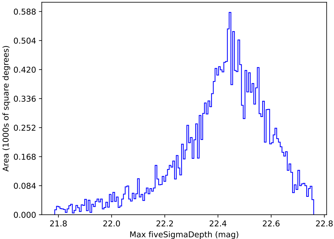
too_ignore_100_1v3.4_10yrs Yr 1 y band: Max fiveSigmaDepth
