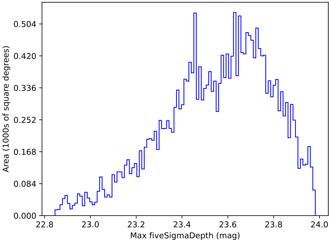
too_ignore_100_1v3.4_10yrs Yr 1 u band: Max fiveSigmaDepth
