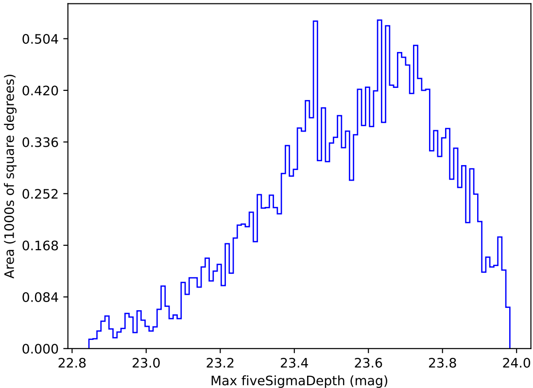
too_ignore_100_1v3.4_10yrs Yr 1 u band: Max fiveSigmaDepth
