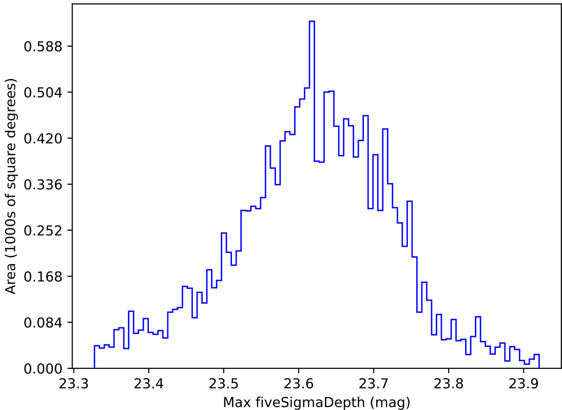
too_ignore_100_1v3.4_10yrs WFD z band: Max fiveSigmaDepth
