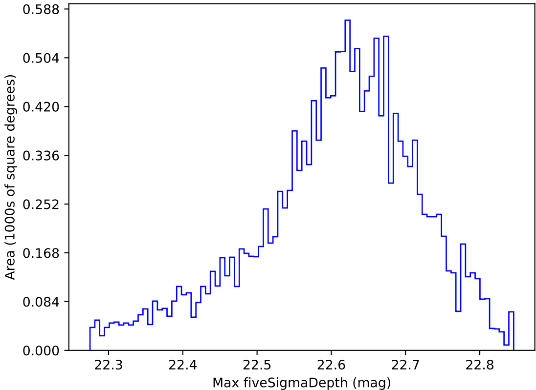
too_ignore_100_1v3.4_10yrs WFD y band: Max fiveSigmaDepth
