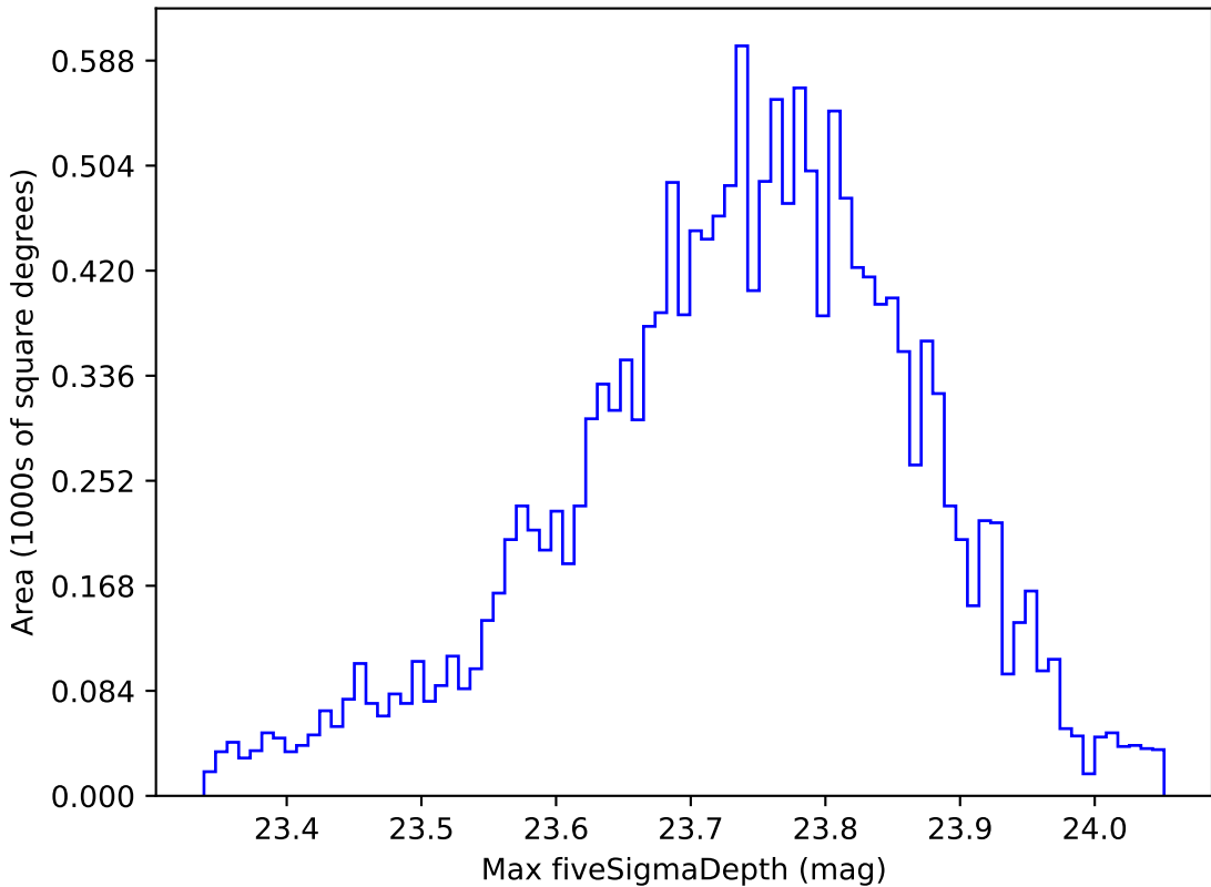
too_ignore_100_1v3.4_10yrs WFD u band: Max fiveSigmaDepth
