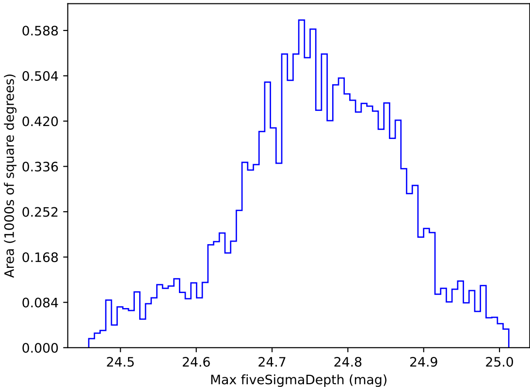
too_ignore_100_1v3.4_10yrs WFD r band: Max fiveSigmaDepth
