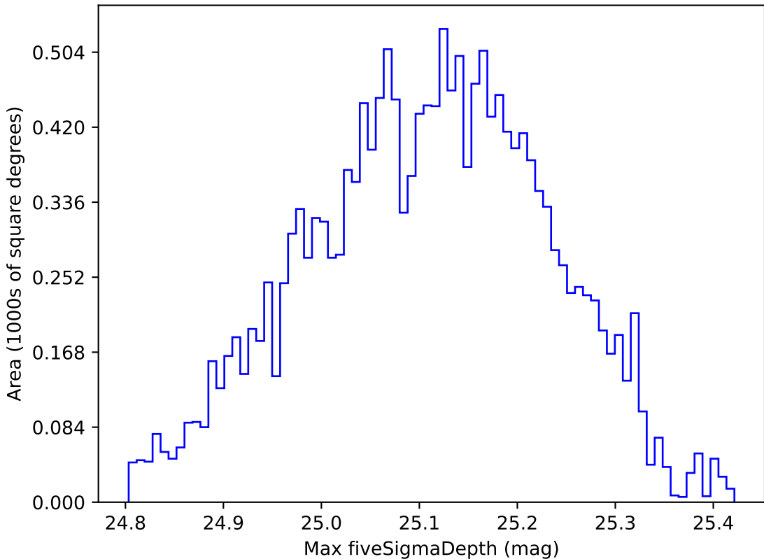
too_ignore_100_1v3.4_10yrs WFD g band: Max fiveSigmaDepth
