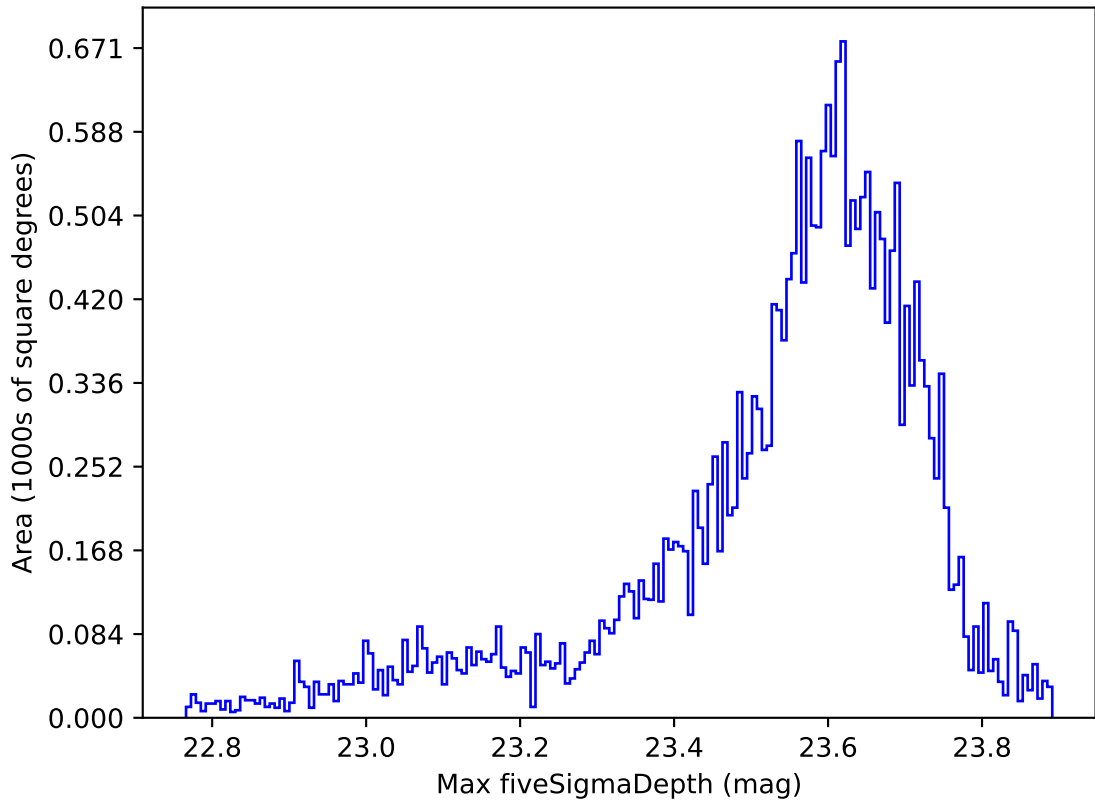
too_ignore_100_1v3.4_10yrs All sky z band: Max fiveSigmaDepth
