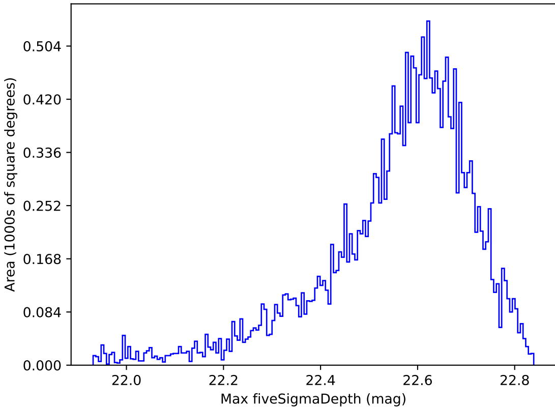
too_ignore_100_1v3.4_10yrs All sky y band: Max fiveSigmaDepth
