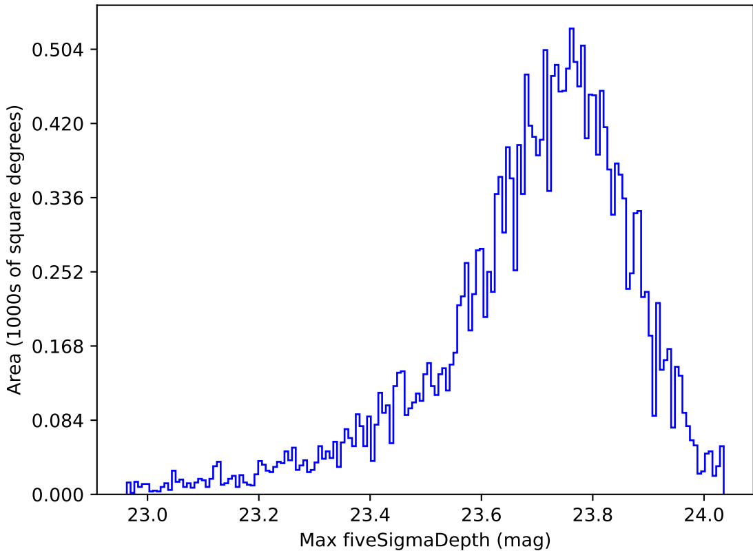
too_ignore_100_1v3.4_10yrs All sky u band: Max fiveSigmaDepth
