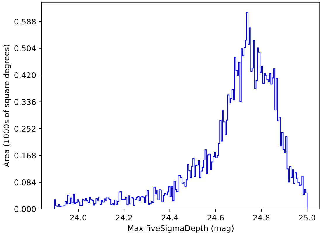
too_ignore_100_1v3.4_10yrs All sky r band: Max fiveSigmaDepth
