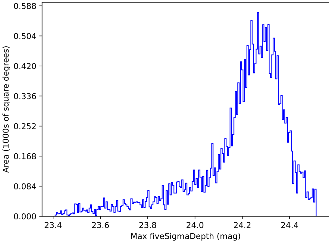
too_ignore_100_1v3.4_10yrs All sky i band: Max fiveSigmaDepth
