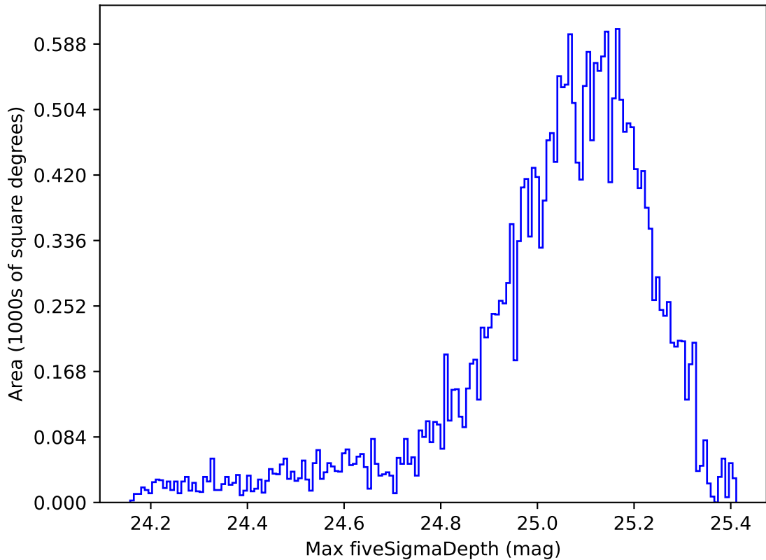
too_ignore_100_1v3.4_10yrs All sky g band: Max fiveSigmaDepth
