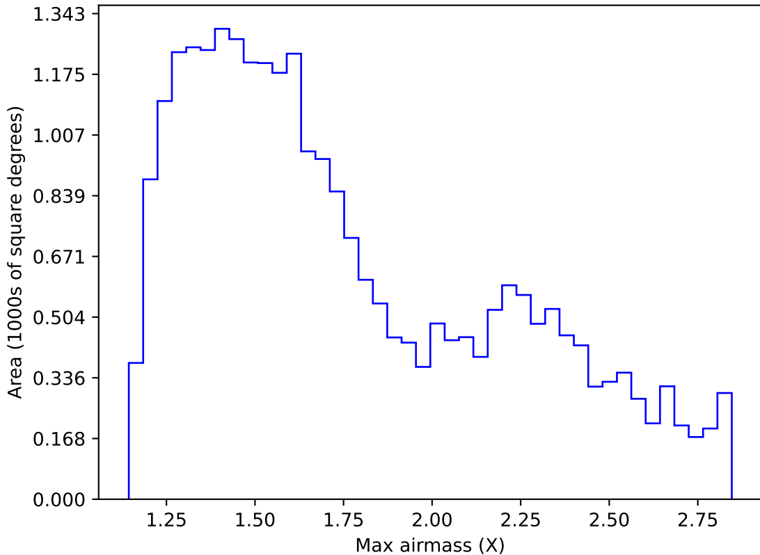
too_ignore_100_1v3.4_10yrs Yr 1 z band: Max airmass
