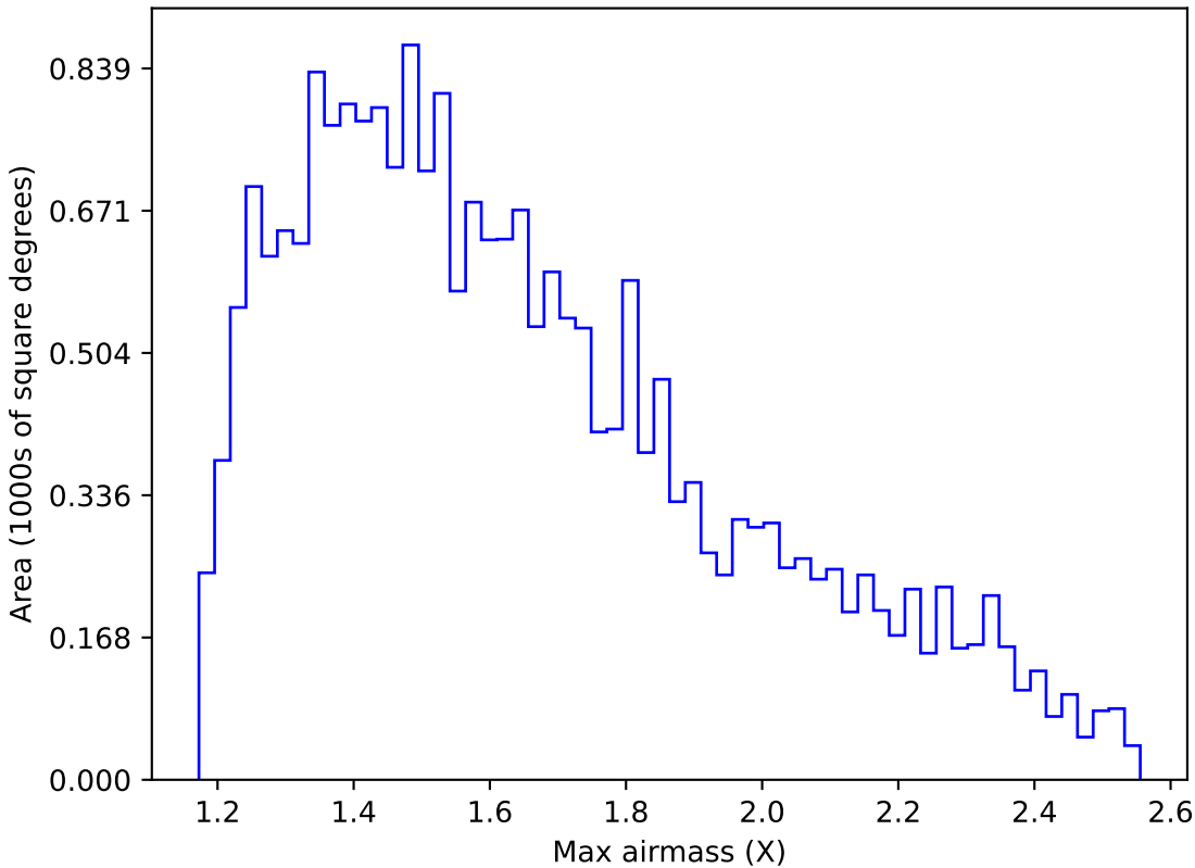
too_ignore_100_1v3.4_10yrs Yr 1 y band: Max airmass
