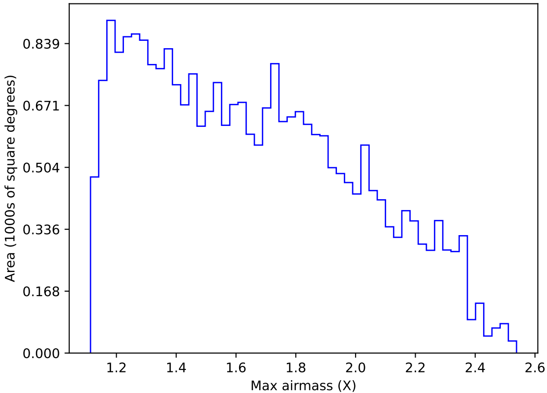
too_ignore_100_1v3.4_10yrs Yr 1 g band: Max airmass
