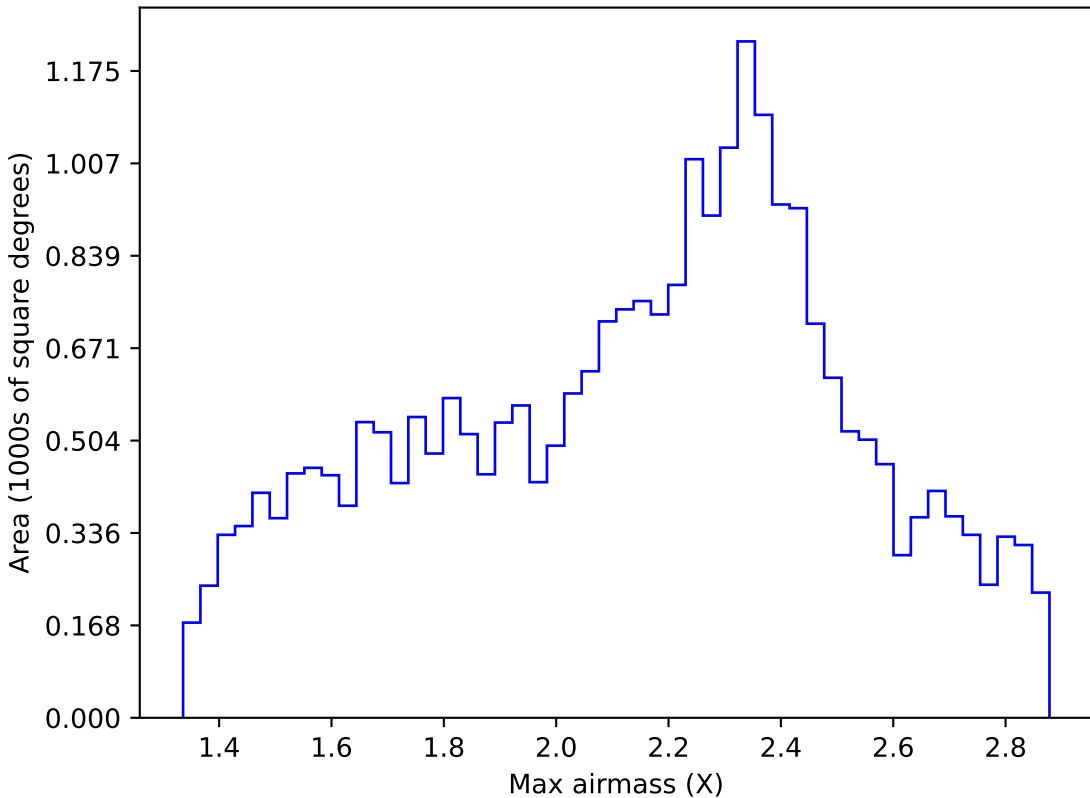
too_ignore_100_1v3.4_10yrs Yr 1 all bands: Max airmass
