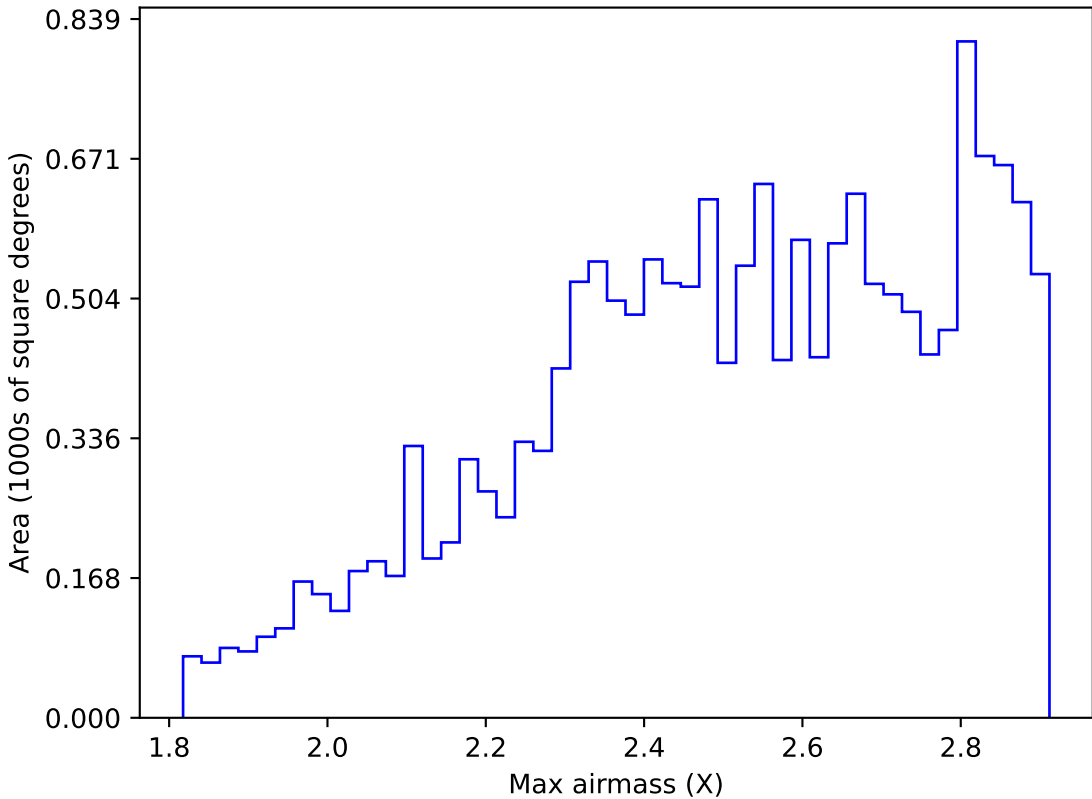
too_ignore_100_1v3.4_10yrs WFD z band: Max airmass
