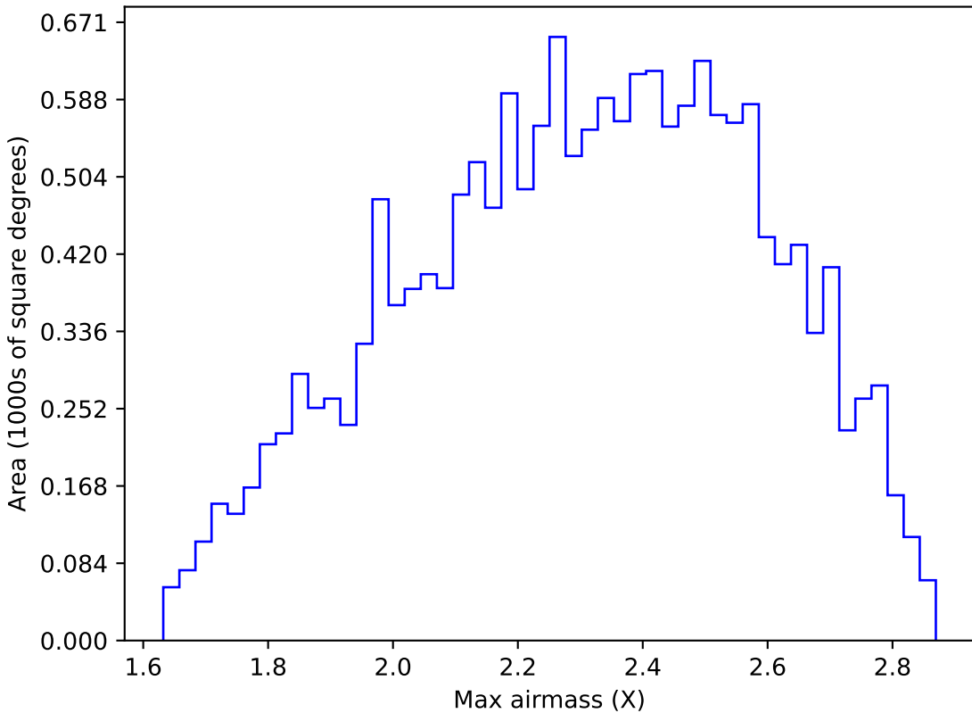
too_ignore_100_1v3.4_10yrs WFD y band: Max airmass
